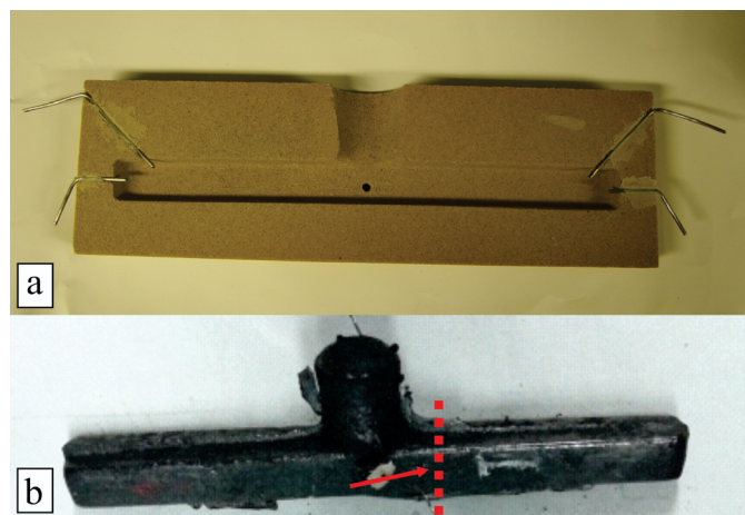
Fig. 1. Measuring cell (a) and a cast sample with marked position of metallographic observations
