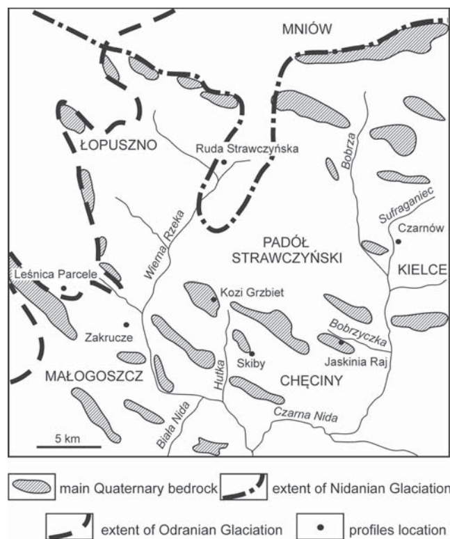
Fig. 2. Location of the cited sections in relation to the maximum extents of the Nidanian and Odranian glaciations in the western part of the Holy Cross Mountains.
