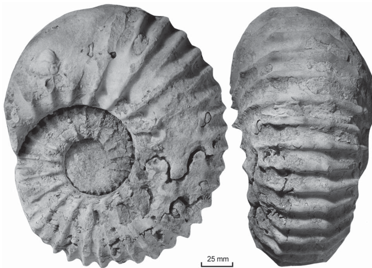
Text-fig. 31. Calycocheras (Newboldiceras) asiaticum spinosum (Kossmat, 1897). OUM KY3433, an incomplete macroconch, with a maximum preserved diameter of 220 mm, from the Karai Formation, Middle Cenomanian asiaticum Zone, section R–S, between Odiyam and Kunnam, at the 1 m level
