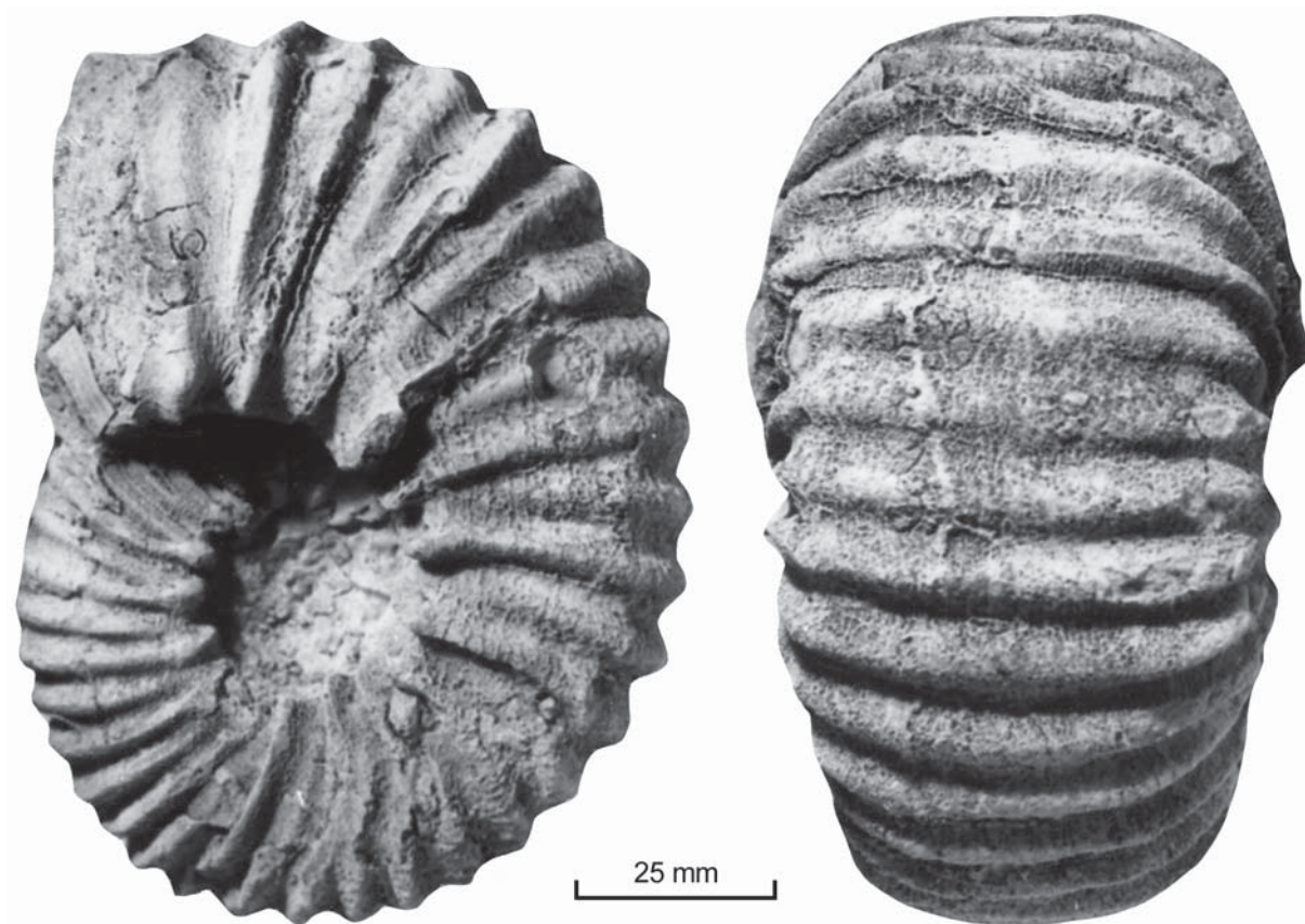
Text-fig. 22. Calycocheras (Calycocheras) naviculare (Mantell, 1822). OUM KY4080, from the Karai Formation, Upper Cenomanian, harpax Zone, from section A, north-west of Garudamangalam at the 9 m level
