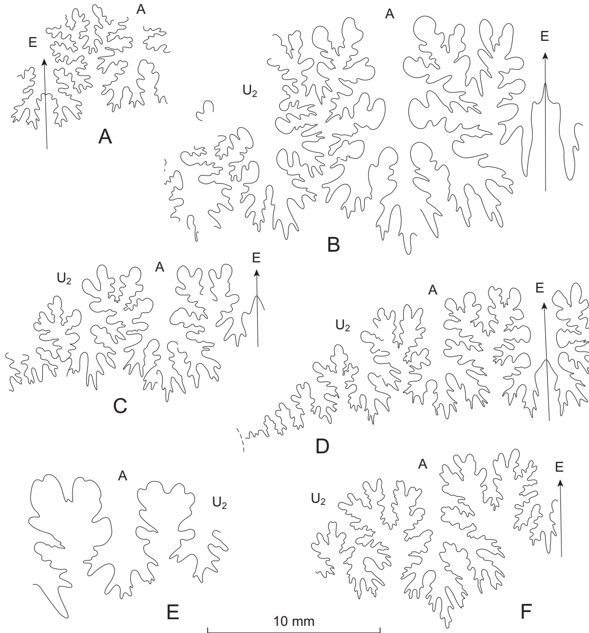
Text-fig. 13. Suture lines: A – Anagaudryceras multiplexum (Stoliczka, 1865), OUM KY2890/3. B – Phylloceras ( Hypophylloceras ) seresitense seresitense (Pervinquière, 1907), OUM KY3732. C – Phylloceras ( Hypophylloceras ) ellipticum Kossmat, 1895, OUM KY4092. D – Phyllopachyceras whiteavesi (Kossmat, 1897), OUM KY3666. E – Algericeras ( Algericeras ) besairiei (Collignon, 1964), OUM KY3666. F – Puzosia ( Puzosia ) compressa Kossmat, 1898, OUM KY2556
