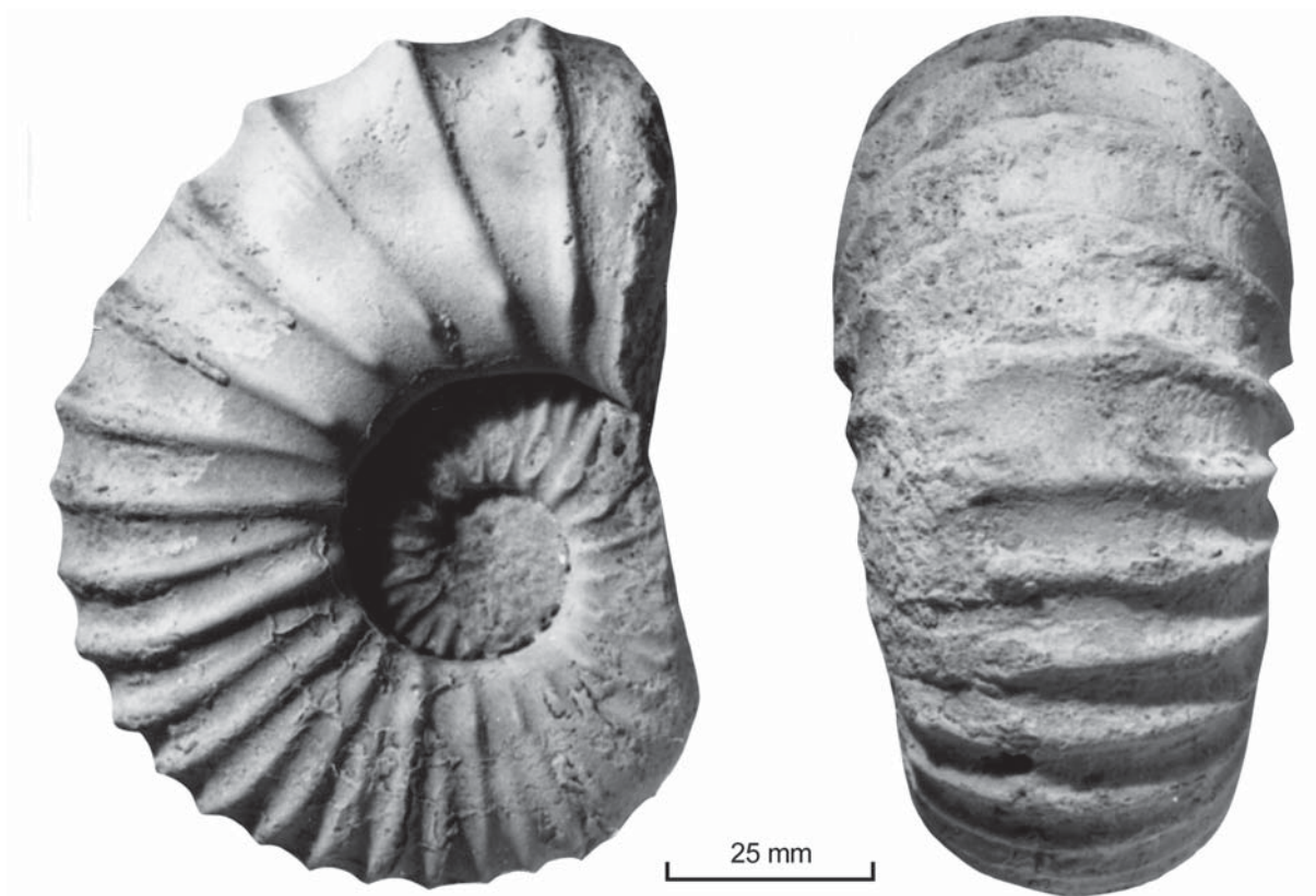
Text-fig. 24. Calycoceras ( Gentoniceras ) boehmi (Spath, 1926b). OUM KY2776, interpreted as an adult microconch, 115 mm in diameter, from the Karai Formation, Middle Cenomanian asiaticum Zone, section K–L, between Odiyam and Kunnam, at the 50–60 m level
