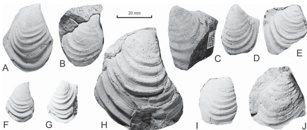
Text-fig. 50. A-D, F, G – Inoceramus chipionkari sp. nov. A – the holotype, OUM KY3362; B – paratype OUM KY3360; C – paratype OUM KY3361; D – paratype OUM KY3359; F – paratype OUM KY3580; G – paratype OUM KY3582; A-D are from section O–P at the 261 m level, Upper Cenomanian septemseriatum Zone; F and G are from section R–S at the 65 m level, Upper Cenomanian, Hourciceras latelobatum – Pseudaspidoceras hourcqi fauna. E, I, J – Inoceramus cf. kamuy Matsumoto and Asai, 1996. E – OUM KY3584; I – OUM KY3583; J – OUM KY3582; all are from section R–S at the 65 m level, Upper Cenomanian, Hourciceras latelobatum – Pseudaspidoceras hourcqi fauna. H – Inoceramus sp. B. OUM KY4548, Upper Cenomanian harpax Zone section R–S, at the 28 m level. All specimens are from the Karai Formation between Odiyam and Kunnam
