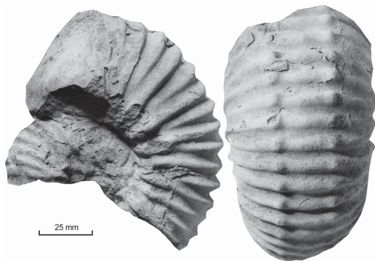
Text-fig. 21. Calycoceras (Calycoceras) naviculare (Mantell, 1822). OUM KY3493, from the Karai Formation, Upper Cenomanian, harpax Zone, section R–S, between Odiyam and Kunnam, at the 19 m level
