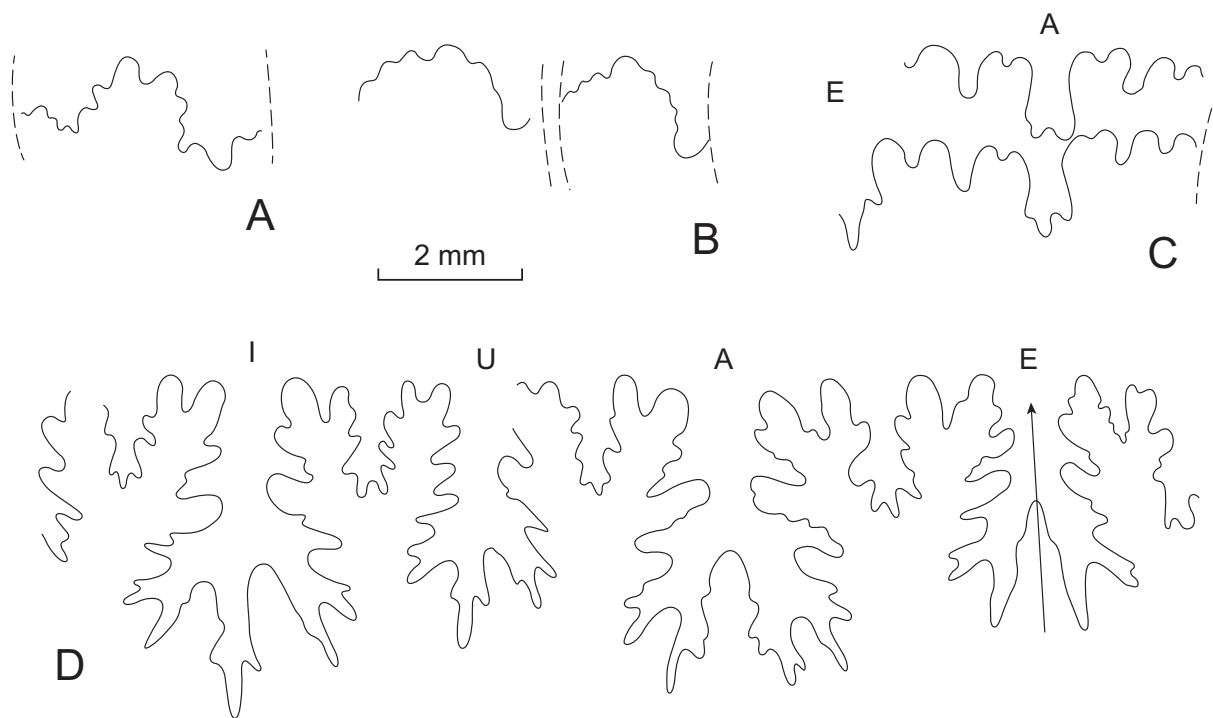
Text-fig. 38. Sutures: A – Carthaginites sp., OUM KY4122. B – Carthaginites multituberculatus sp. nov., OUM KY3913. C – Worthoceras sp., OUM KY4202. D – Hemiptychoceras cf. tropicum (Kossmat, 1895), OUM KY3699a
