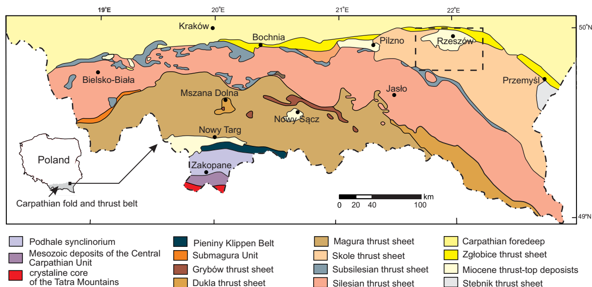
Text-fig. 1. Simplified geological map of the Polish part of the Carpathians based on Oszczytko et al. (2008), modified. The dashed box shows the study area
