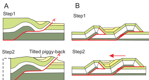
Text-fig. 4. Models of thrust-top basin sedimentation. A – Roure et al. (1991); B – Bonini et al. (1999)
