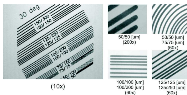
Fig. 5. Test pattern on PCB after etching process
