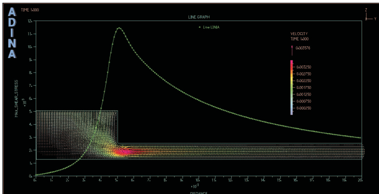
Fig. 13. Finite element modeling of the cell detachment experiment
