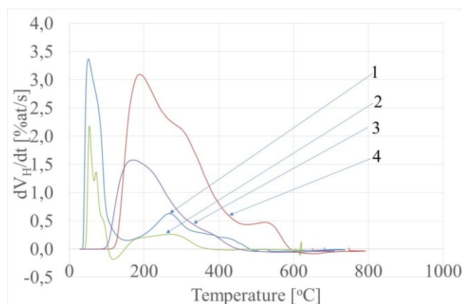
Fig. 7. Changes in hydrogen content in gases evolved during casting of ductile iron related to the mould temperature: 1) casting thickness 13 mm, sand with the SL resin, 2) casting thickness 13 mm, sand with the SL 2002 resin, 3) casting thickness 40 mm, sand with the SL resin, 4) casting thickness 40 mm, sand with the SL 2002 resin
