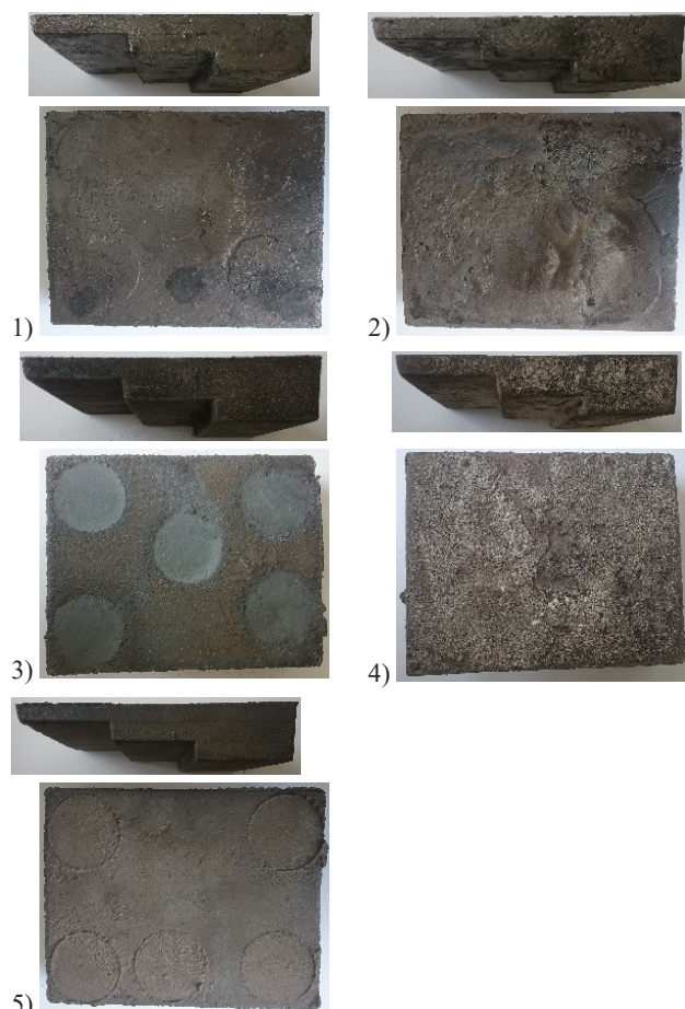
Fig. 3. Sample ductile iron castings during direct gas evolution test. Castings made in sand moulds with: 1) SL resin, 2) SL 2002 resin, 3) furan resin, 4) bentonite and coal dust, 5) Besil binder
