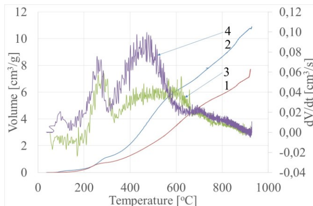
Fig. 10 Gas forming tendency and its changes observed in the sand with: 1) SL resin, 2) SL2002 resin, 3) SL resin (instantaneous values), 4) SL2002 resin (instantaneous values)
