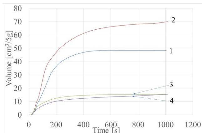
Fig. 9. Gas volume released during heating up 5 grams of the sand with: 1) SL resin, 2) SL2002 resin, 3) SL resin (reheating), 4) SL2002 resin (reheating)
