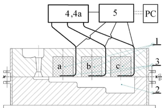
Fig. 1. Test stand for direct measurement of gas evolution rate from moulding sands: 1) mould elements (height of mould cavity under the measuring point: a-13 mm, b-26 mm, c-40 mm), 2) mould cavity with the gating system, 3) gas sampling location, 4) and 4a) gas sensors, 5) Agilent recorder [8, 9]
