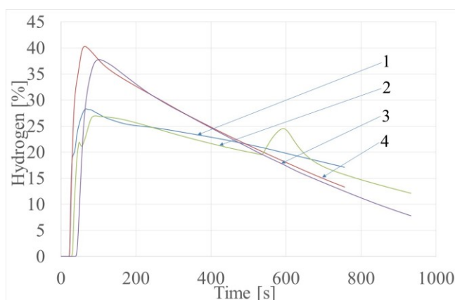
Fig. 6. Hydrogen content in gases evolved during casting of ductile iron: 1) casting thickness 13 mm, sand with the SL resin, 2) casting thickness 13 mm, sand with the SL 2002 resin, 3) casting thickness 40 mm, sand with the SL resin, 4) casting thickness 40 mm, sand with the SL 2002 resin
