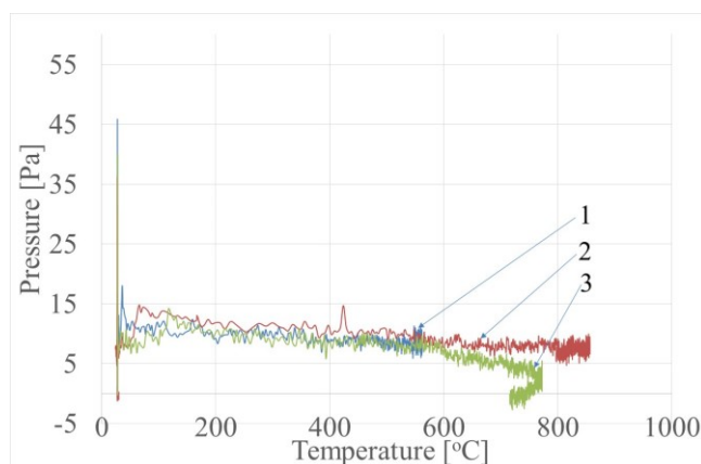
Fig. 4. Pressure of gases released from mould with the SL2002 resin during pouring of ductile iron castings with the wall thickness: 1) 13 mm, 2) 26 mm, 3) 40 mm
