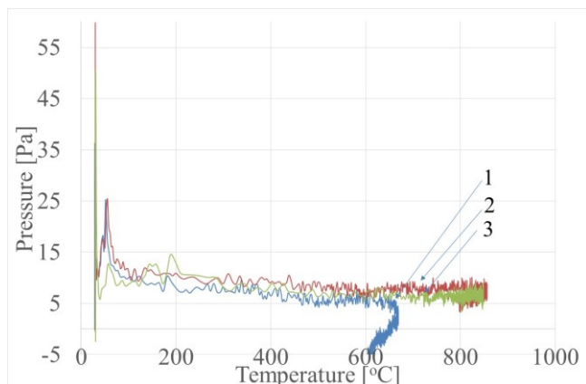
Fig. 5. Pressure of gases released from mould with the SL resin during pouring of ductile iron castings with the wall thickness: 1) 13mm, 2) 26mm, 3) 40mm
