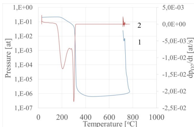
Fig. 8. Oxygen content in gases evolved during casting of ductile iron related to the mould temperature: 1) partial pressure, 2) changes in pressure
