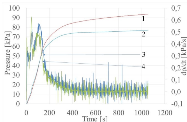
Fig. 11 Pressure of gases and increase in this pressure during gas evolution test: 1) pressure for sand with the SL resin, 2) pressure for sand with the SL 2002 resin, 3) pressure increase for sand with the SL resin, 4) pressure increase for sand with the SL 2002 resin
