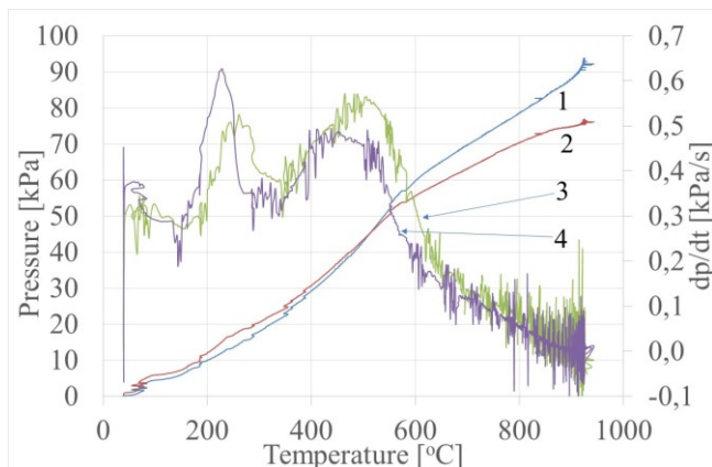
Fig. 12. Temperature-related pressure of gases and changes in this pressure during gas evolution test: 1) pressure for sand with the SL resin, 2) pressure for sand with the SL 2002 resin, 3) pressure increase for sand with the SL resin, 4) pressure increase for sand with the SL 2002 resin
