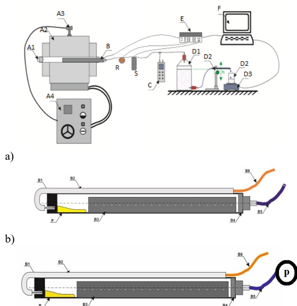
Fig. 2. Schematic diagram of the test stand for indirect gas evolution measurement [7] showing measuring flasks used in: a) volumetric method [7], b) pressure-assisted method
