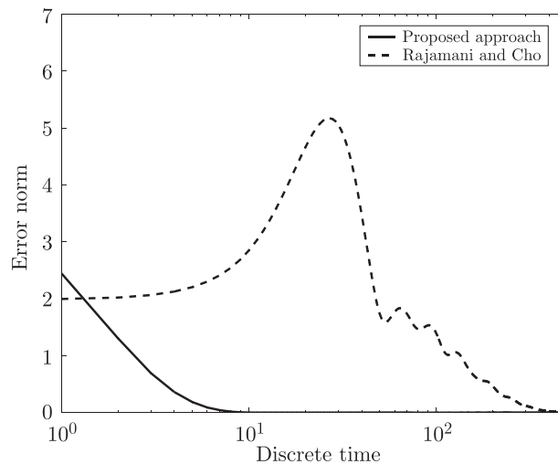
Fig. 5. Norm of the state estimation error \|e_k\|_2
