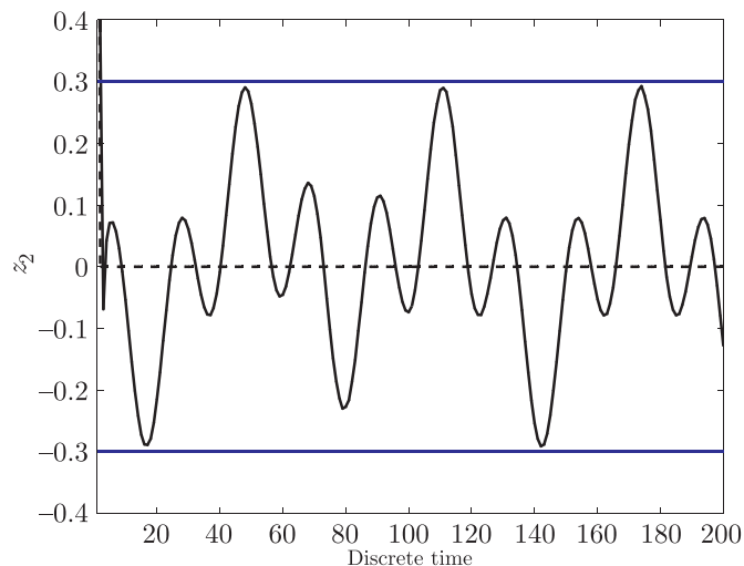
Fig. 7. Residual z_{2,k} = y_{2,k} - \hat{y}_{2,k} obtained with the UIO (dashed line) and the conventional observer
