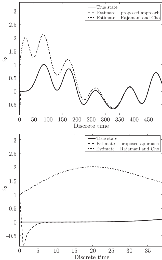
Fig. 3. Angular position of the link x_3 and their estimates
