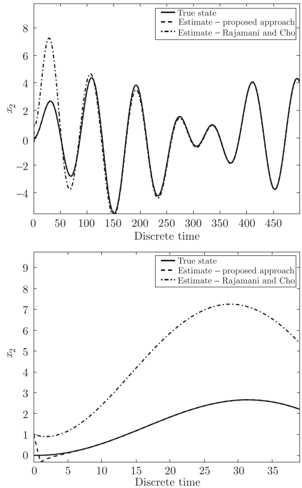
Fig. 2. Angular velocity of the motor x_2 and their estimates
