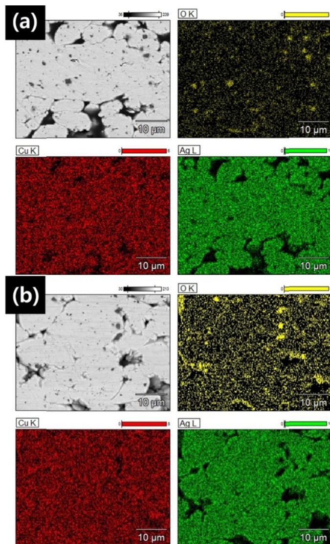
Fig. 8. EDS mapping results of mechanically alloyed Ag-40Cu particles sintered at 10 MPa for 10 min at different temperatures: (a) 225°C and (b) 250°C
