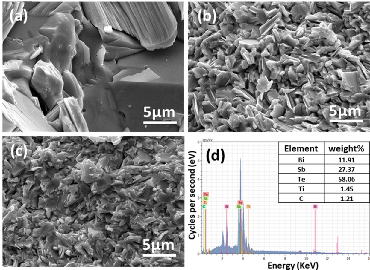
Fig. 3. Fracture surface of (a) BiSbTe/0 wt.% TiC, (b) BiSbTe/1 wt.% TiC and (c) BiSbTe/2 wt.% TiC nanocomposite bulk samples and (d) EDS mapping analysis for the BiSbTe/2 wt.% TiC nanocomposite sample
