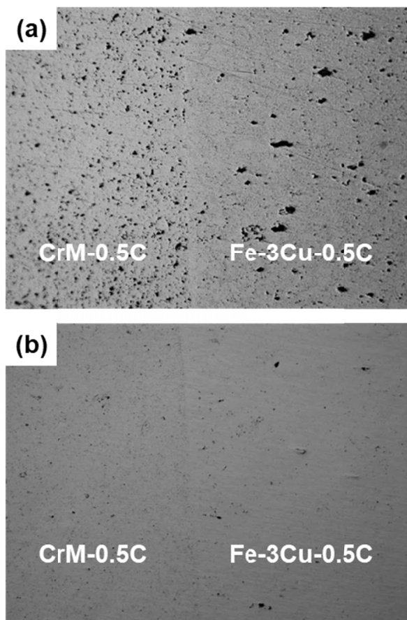
Fig. 3. Un-etched micrographs of interfacial region between high- and low-alloys when secondarily compacted with (a) 500 MPa and (b) 700 MPa
