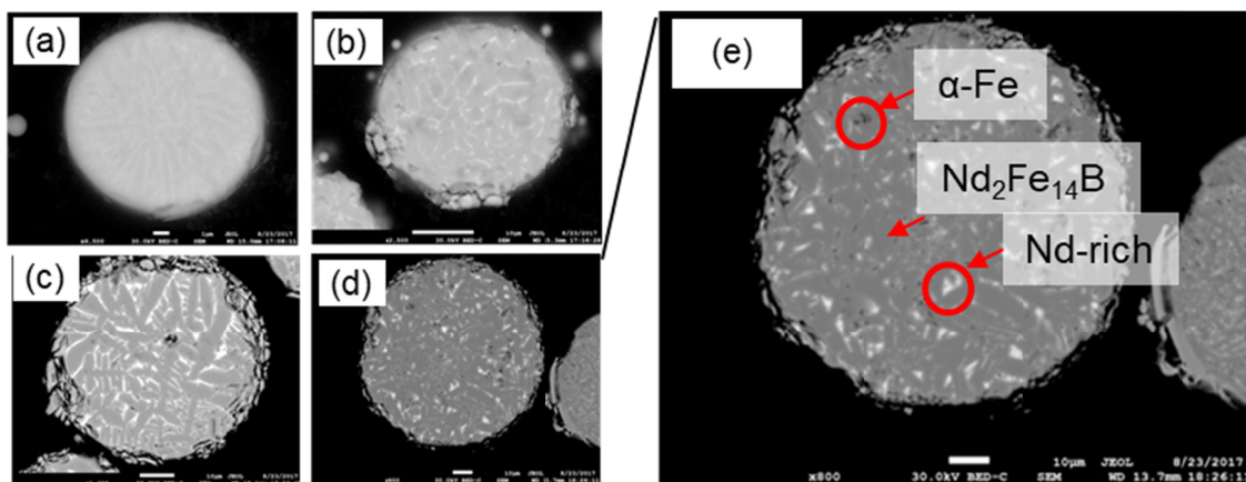
Fig. 1. Microstructure of atomized Nd-Fe-B powder with powder size (a) 10\ \mu\text{m} , (b) 30\ \mu\text{m} , (c) 60\ \mu\text{m} , (d) 90\ \mu\text{m} and (e) enlarged 90\ \mu\text{m} respectively; Nd-rich (white), \text{Nd}_2\text{Fe}_{14}\text{B} (gray) and \alpha -Fe (dark)
