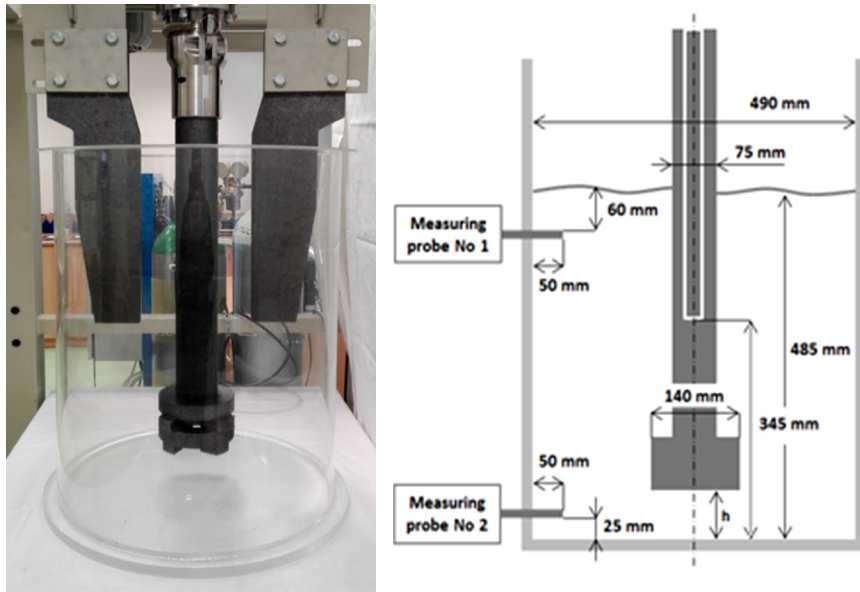
Fig. 1. Physical model of the refining ladle and its dimensions [12]
