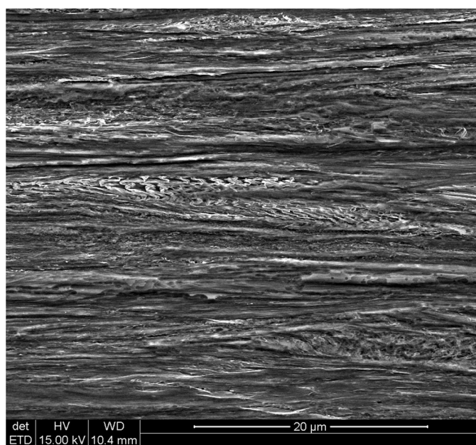
Fig. 4. Microstructure from regions close to the axis of final \phi 1.7 mm-diameter wire drawn in conventional drawing dies at a speed of v = 20 m/s; G_c = 90.5\% ; a longitudinal microsection
