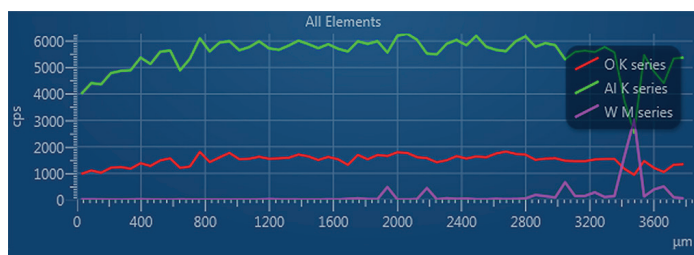
Fig. 10. EDS Linescan results through the zones of Al_2O_3 -W (measurements line at Fig. 9)
