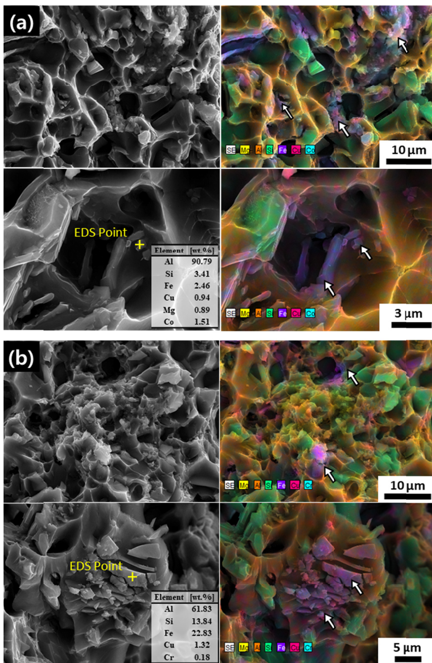
Fig. 6. Scanning electron micrograph and EDS-mapping was observed on fracture surface of extruded Al-12.6Si-3Cu-0.6Mg-0.5Fe-0.5X [X = (a) : Co, (b) : Cr] alloys
