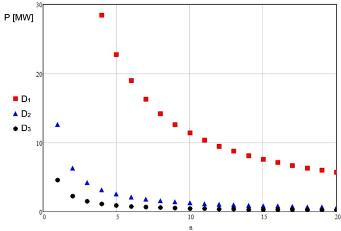
Fig. 15. Power consumption of each coil.
