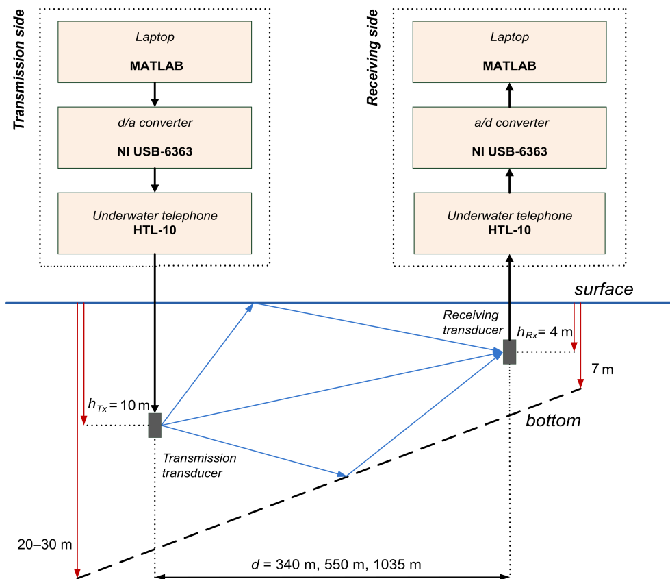
Fig. 3. Measuring system.
