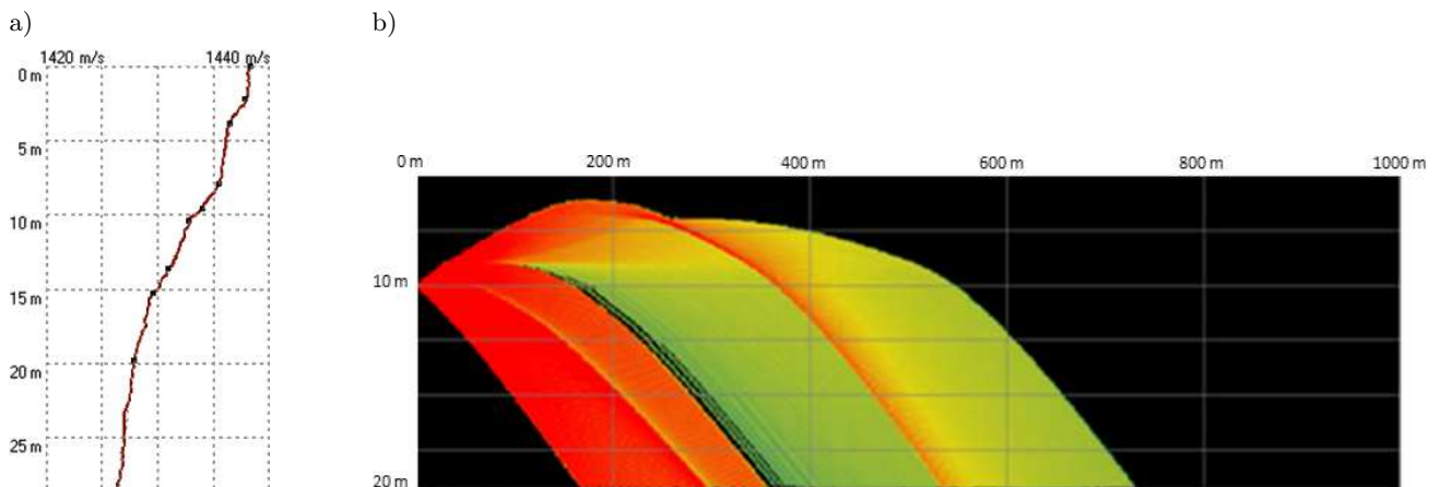
Fig. 4. Measured sound speed profile (a) and estimated range (b).
