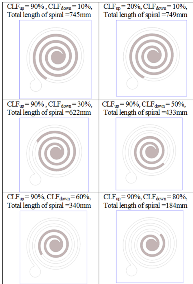
Fig. 10. Castability trial, simulation results (Cast Iron GJL 250, T_{pouring} = 1348^{\circ}C , green sand moisture = 3,3%) – sensitivity test of simulation results (obtained length of the spiral) on the variation of CLF_{up} CLF_{down}
