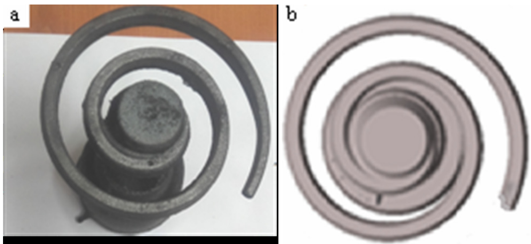
Fig. 9. Castability trial (spiral shape) – validation result (GJL 250, T_{pouring} = 1348^{\circ}\text{C} , green sand moisture = 3,3%), a. experiment, b. simulation result (CLF up = 90%, CLF down = 60%)
