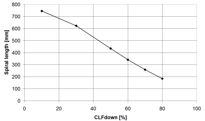
Fig. 11. Sensitivity test of simulation results (obtained length of the spiral) on the changes of CLF_{down} (Cast Iron GJL 250, T_{pouring} = 1348^{\circ}C , green sand moisture = 3,3%)
