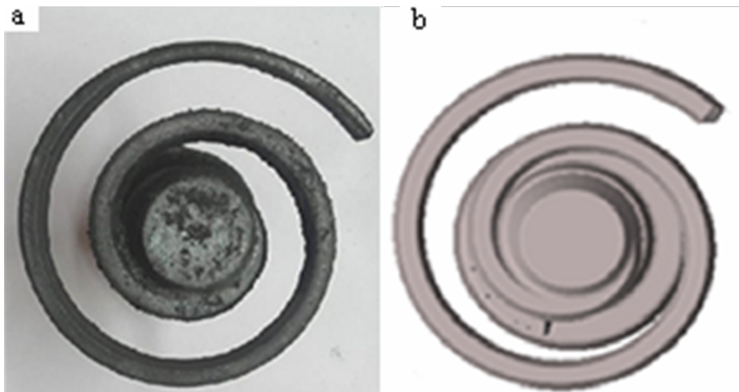
Fig. 8. Castability trial (spiral shape) – validation result (GJL 250, T_{pouring} = 1348^{\circ}\text{C} , green sand moisture = 6,6%), a. experiment, b. simulation result (CLF up = 90%, CLF down = 60%)
