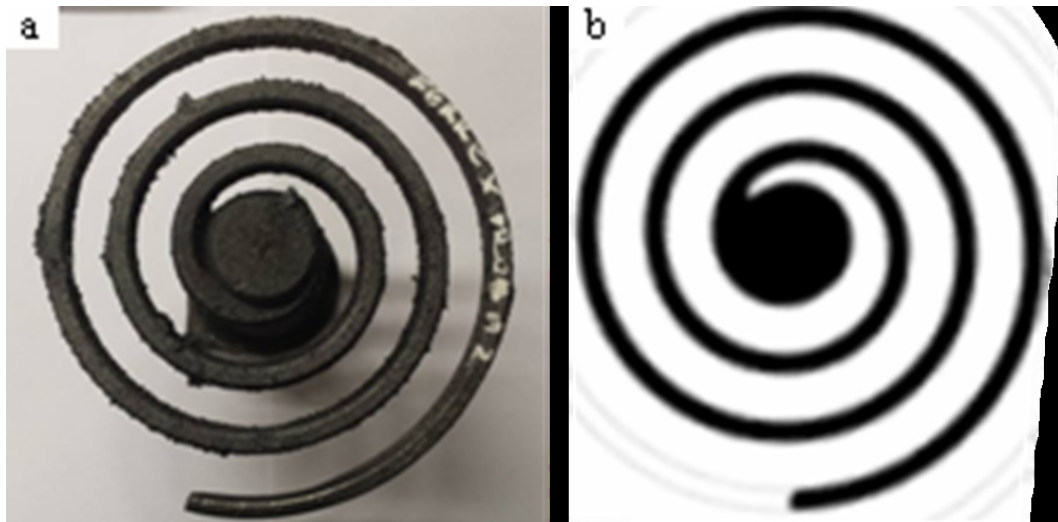
Fig. 7. Castability trial (spiral shape) – validation result (GJS-400-15, T_{pouring} = 1367^{\circ}\text{C} , green sand moisture = 3,3%), a. experiment, b. simulation result (CLF up = 70%, CLF down = 10%)
