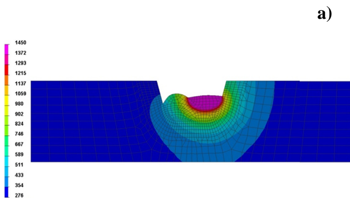
Fig. 5. A calibration example of the heat source model for bead number 4 – view of the temperature distribution on the cross-section of the model a) and geometry of 3rd and 4 th bead b)
