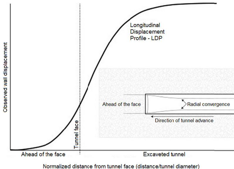
Fig. 11. Use of the longitudinal displacement profile, (LDP), to relate tunnel wall displacement as a function of distance from face (Lato & Diederichs 2014)
