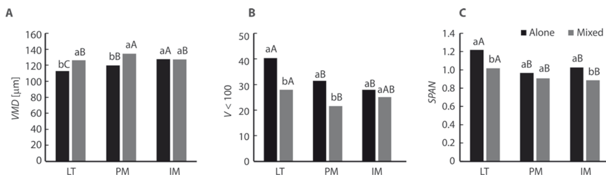
Fig. 1. (A) – Volumetric median diameter ( VMD ), (B) – percentage of the volume of droplets smaller than 100 \mu\text{m} ( V < 100 ) and (C) – coefficient of droplet size uniformity ( SPAN ) for insecticides lambda-cyhalothrin + thiamethoxam (LT), phosmet (PM) and imidacloprid (IM) isolated and combined with acaricide applied with a hollow cone nozzle (TXA 8002). Columns followed by lowercase letters were used to compare insecticide alone and mixed with acaricide, while uppercase letters were used to compare insecticides for alone and mixed spray separately. The same letters do not differ significantly from each other by the Tukey's test ( p > 0.05 )
