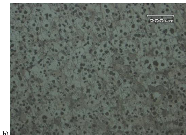
Fig. 8. Micrograph by pouring temperature of 1320 °C; (a) contact section (b) inner part. Etched with 3% Nital
