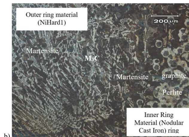
Fig. 11. Micrographs by pouring the inner ring at temperature 1410 °C; (a) nodular cast iron in outer and inner ring cavities; (b) direct contact inner and outer ring material. Etched with Nital 3%.
