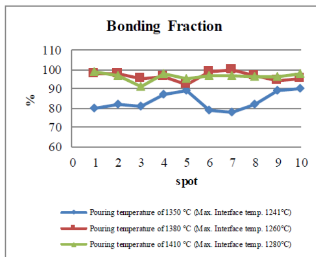
Fig. 16. The bonding fraction of the interface plate to the inner ring at various pouring temperature
