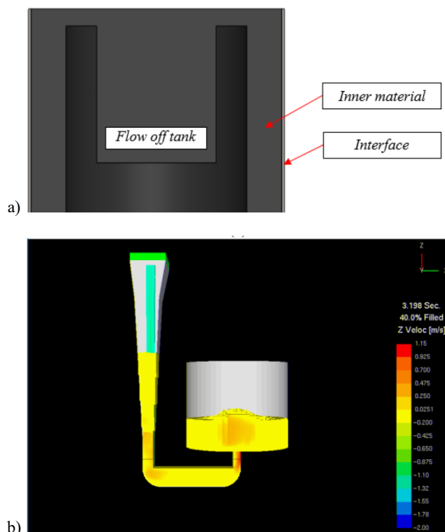
Fig. 2. Schematic of flow-off tanks as initial heater interfaces (a) and SolidCAST simulation (b)
