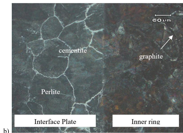
Fig. 9. Micrographs of the contact area interface-inner ring by pouring temperature of 1350 °C; (a) contact section; (b) inner parts. Etched with 3% Nital
