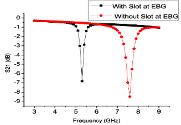
Fig. 2. Comparison of S_{21} versus frequency plot of conventional mushroom-type EBG structure and C-slotted mushroom-type EBG structure
