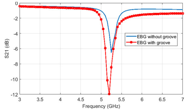
Fig. 4. Frequency response of the S_{21} parameter without and with a groove coupled EBG in the microstrip line
