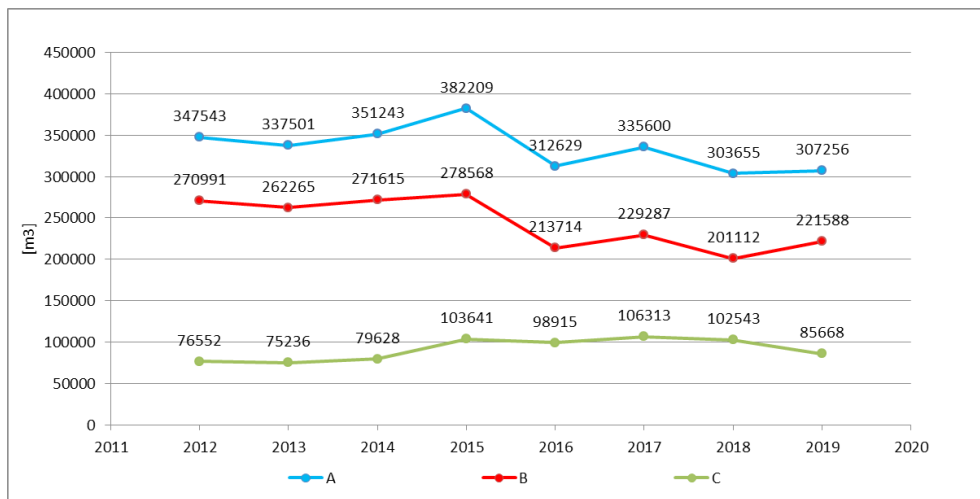
Fig. 2. A – Geothermal water production in the Mszczonów IG-1 well, B – The use of geothermal waters in the geothermal plant for heating purposes, C – The use of geothermal water in the recreation centre Termy Mszczonów
