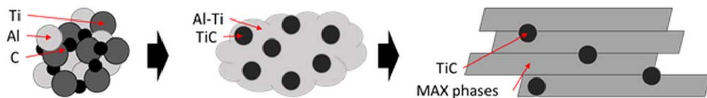
Fig. 5. Formation mechanism of MAX phases in Ti-Al-C system [27]
