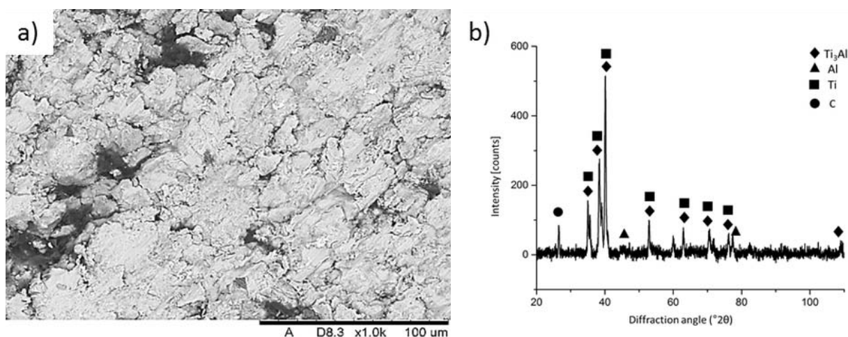
Fig. 6. SPS products for sintering temperature of 700^\circ C : a) microstructure, b) XRD analysis
