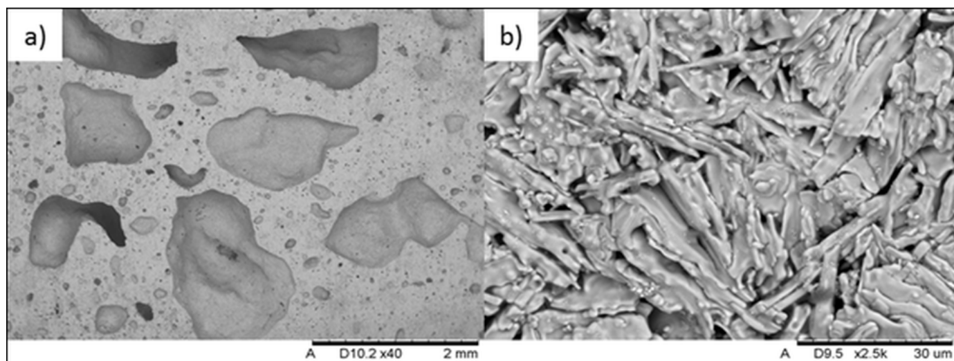
Fig. 1. Manufactured MAX phase preform: a) view of the overall open porosity, b) microstructure of MAX phase platelets
