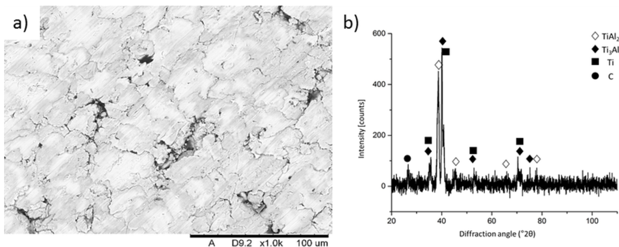
Fig. 7. SPS products for sintering temperature of 850^\circ C : a) microstructure, b) XRD analysis
