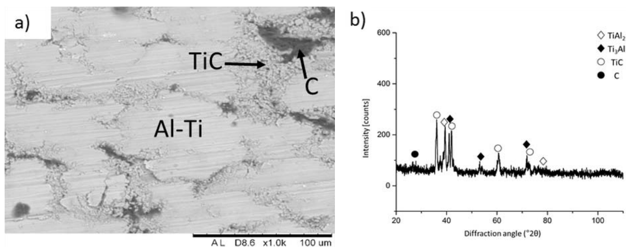
Fig. 4. SPS products for sintering temperature of 1250°C: a) microstructure, b) XRD analysis
