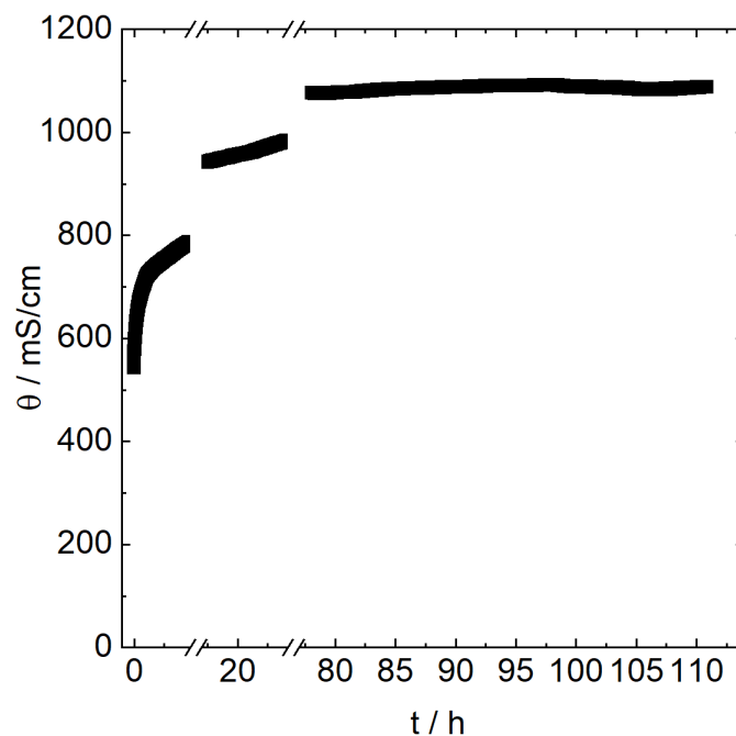
Fig. 9. Conductivity of the acidic solution during dissolution of raw \text{BiVO}_4 ( \text{H}_2\text{SO}_4 , \text{pH} = 3 , T = 19^\circ\text{C} )
