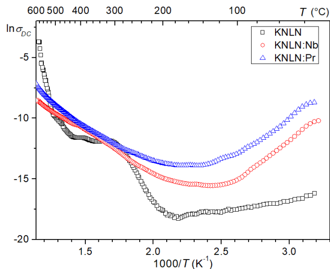
Fig. 5 The \ln\sigma_{DC}(1/T) relationship for the KNLN type materials
