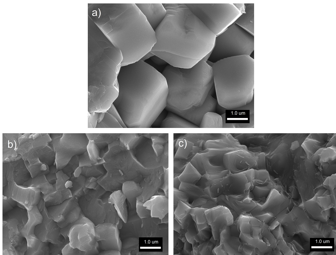
Fig. 3. SEM images of the KNLN (a), KNLN:Nd (b) and KNLN:Pr (c) materials
