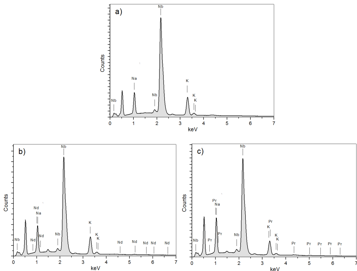
Fig. 4. EDS tests of the (a) KNLN, (b) KNLN:Nd and (c) KNLN:Pr materials
