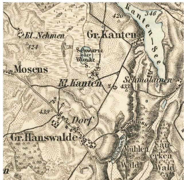
Fig. 2. Location of the Lake Mlynek (Mühlchen See), the Lake Kątny (Kanten See), village Janiki Wielkie (Hanswalde), the Prussian stronghold (Schloss), the nearby mill on a stream and the forest around the lake in the second half of the 19th century. Karte des Deutschen Reiches 1:100,000, Christburg, 1893.
