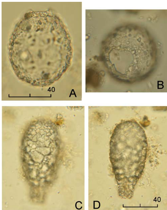
Fig. 6. Agglutinated shell of testate amoebae – A, B Cucurbitella tricuspis , C, D Diffflugia (1.10 cm depth).
