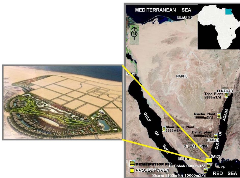
Fig. 5. Site location showing artificial lagoon layout, and desalination plants in South Saini Governorate; source: own elaboration
