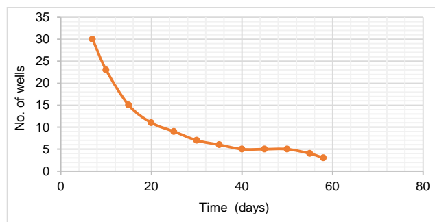
Fig. 18. Relation between the no. of wells and time; source: own study
