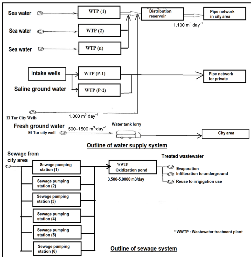
Fig. 4. Outline of the water supply and sewerage system in Sharm El-Sheikh City; source: JICA, WRRRI [1999]
