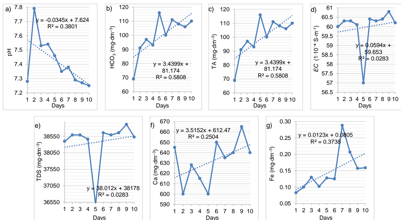
Fig. 19. Water quality analysis for production well No. 5 for chosen physico-chemical parameters: a) pH, b) HCO 3 , c) total alkalinity (TA), d) electrical conductivity (EC), e) total dissolved solids (TDS), f) Ca, g) Fe; source: own study
