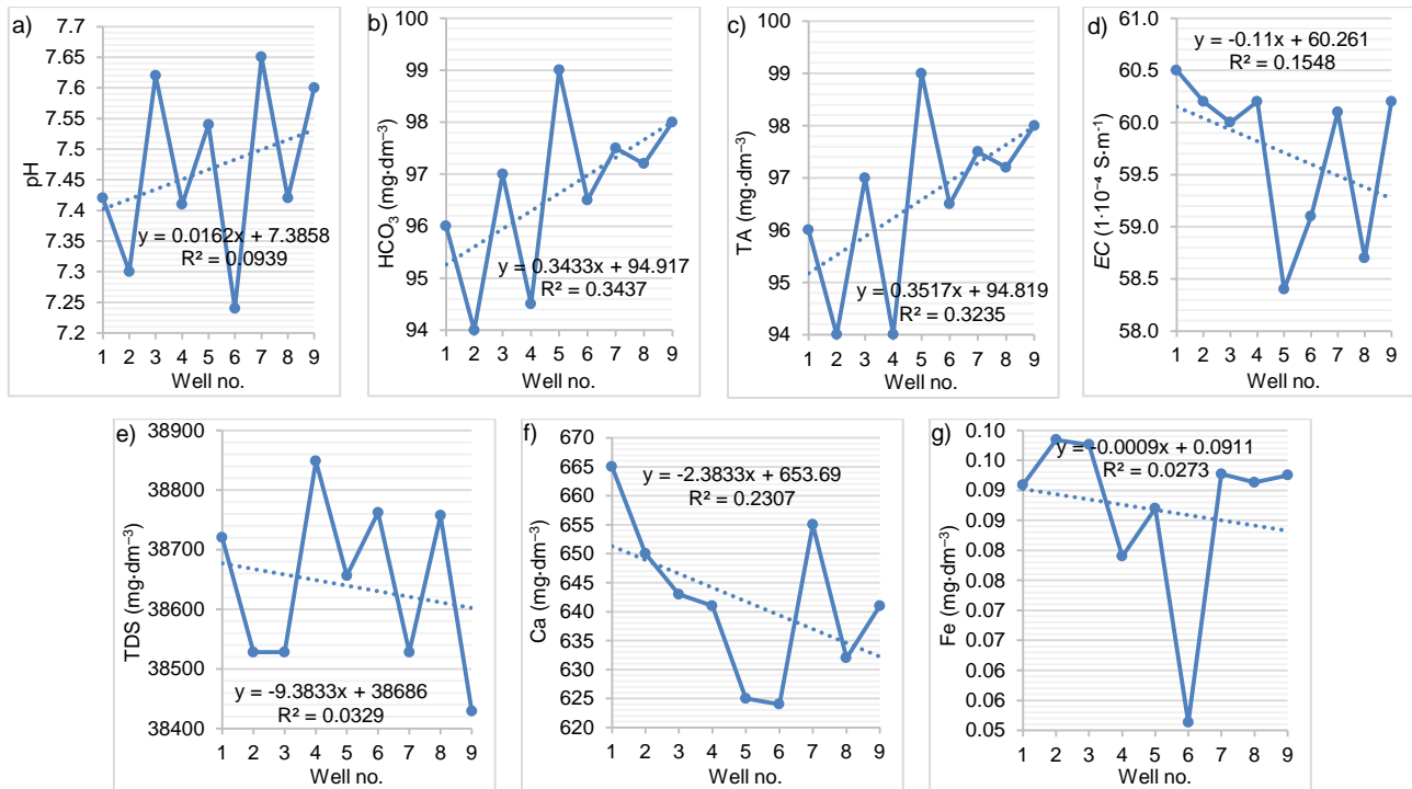
Fig. 20. Analysis of chosen physico-chemical parameters for nine injection wells for the lagoon area: a) pH, b) \text{HCO}_3^- , c) total alkalinity (TA), d) electrical conductivity (EC), e) total dissolved solids (TDS), f) Ca, g) Fe; source: own study
