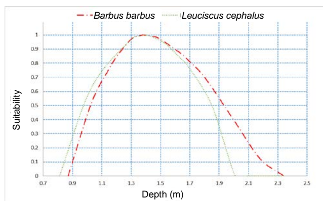
Fig. 2. Habitat suitability curves for individual fish species for depth of the Váh River in the city of Piešťany; source: own study
