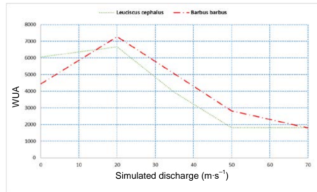
Fig. 3. Weighted usable area (WUA) for individual fish species of the Váh River at different discharge rates
