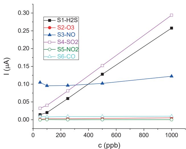
Fig. 4. Sensor responses in given concentrations of SO 2
