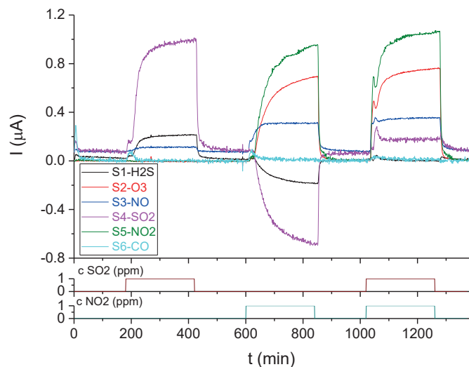
Fig. 7. Sensor responses converted to concentrations
