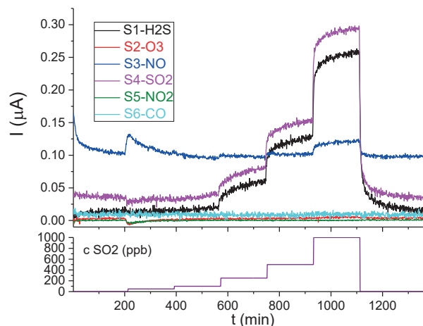
Fig. 2. Sensor response to different concentrations of SO 2
