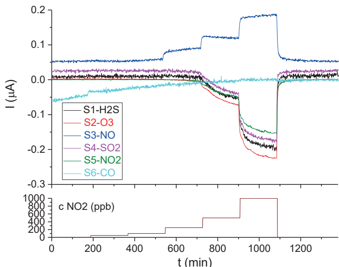
Fig. 3. Sensor response in given concentrations of NO 2
