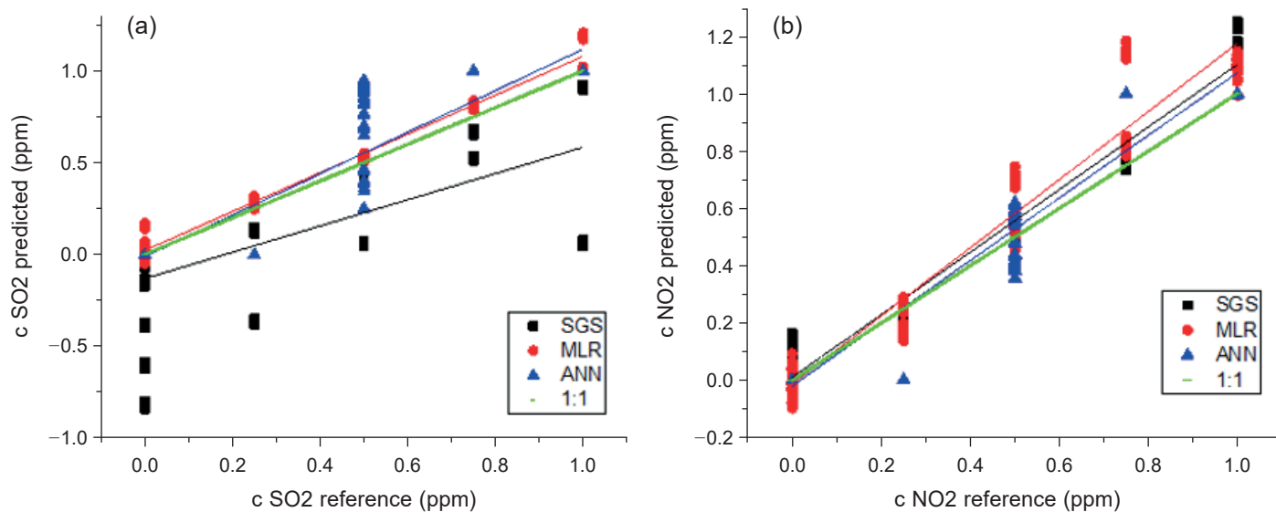
Fig. 8. Predictions of gas concentrations made on a test dataset with the use of SGS, MLR and ANN methods against reference concentrations of: a) \text{SO}_2 , b) \text{NO}_2 with linear regression lines. The training set consisted of only measurements in one toxic gas and synthetic air
