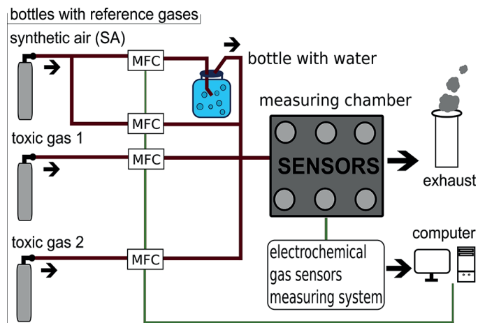
Fig. 1. Structure of the measuring stand
