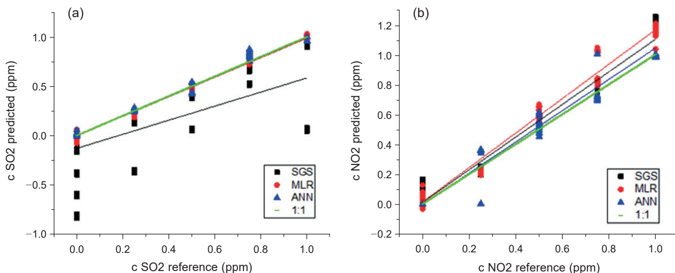
Fig. 9. Predictions of gas concentrations made on test dataset with the use of SGS, MLR and ANN methods against reference concentrations of: a) SO 2 , b) NO 2 with linear regression lines. The training set consisted of measurements in single gas, binary mixture, and synthetic air
