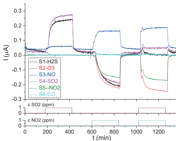
Fig. 6. Raw sensor responses to SO 2 and NO 2
