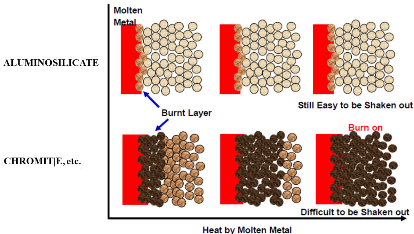
Fig. 4. Comparison of heat resistance of studied sands [12]
