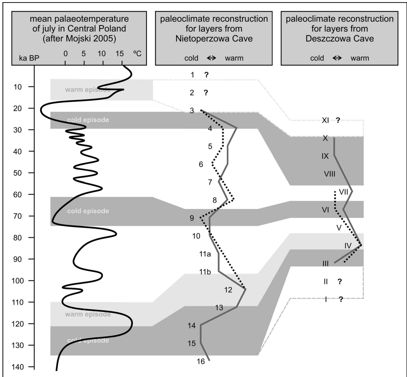
Fig. 8. Correlation of the most distinctive peaks of the palaeotemperature curves reconstructed for sediments of Nietoperzowa Cave and Deszczowa Cave with the palaeoclimatic curve of the late Quaternary of Poland. The numbers next to the curves denote layers of sediments.
