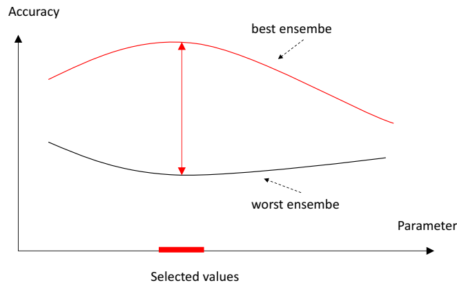
Figure 1 Qualitative illustration of the criterion used for choosing the training set size and the number of hidden units in NN classifiers ( X axis): maximizing the accuracy gap between the best and the worst ensemble of a given size (see text for the details).
