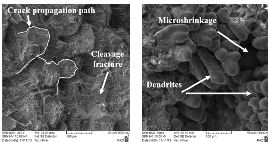
Intergranular brittle fracture
