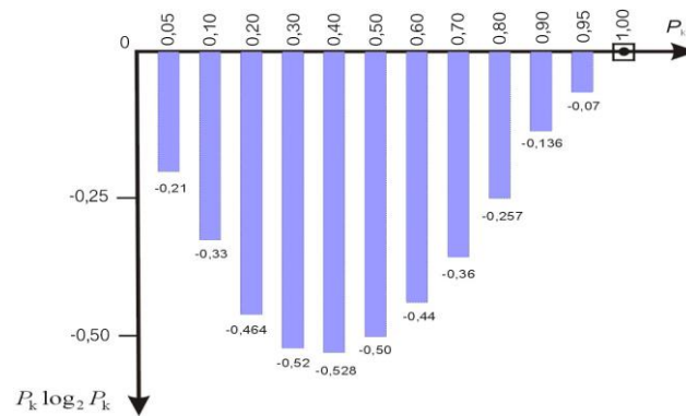
Fig. 3. Information uncertainty k-th state of the event P_k .
