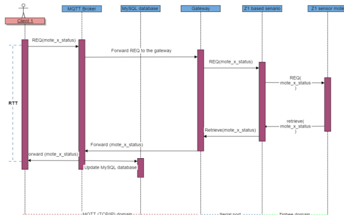
Fig. 6 Message sequence.
