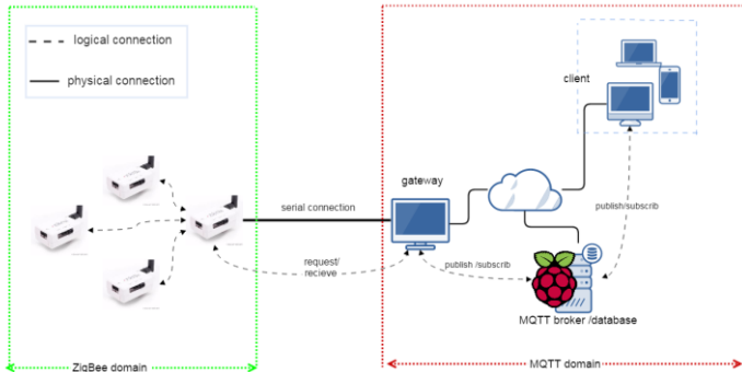
Fig. 5 Network design
