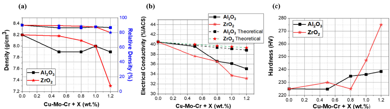
Fig. 4. Physical properties of the Cu-Mo-Cr-X (X = ZrO 2 and Al 2 O 3 ) composite
