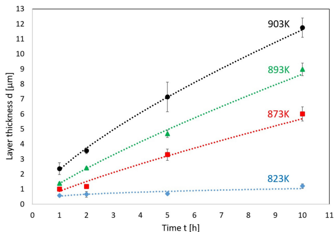
Fig. 4. Dependence of the intermetallic layer's average thickness on the annealing time and temperature
