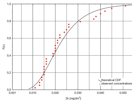
Truncated distribution
