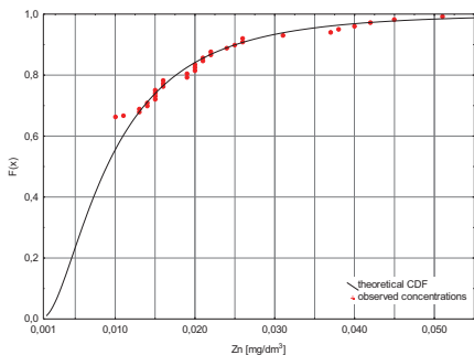
Censored distribution
