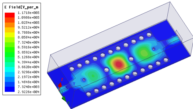
Fig. 8. Simulated E-field magnitude distributions obtained by SIW bandpass filter
