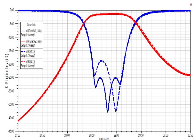
Fig. 10. S-parameters of the proposed SIW bandpass filter with optimal geometric parameters
