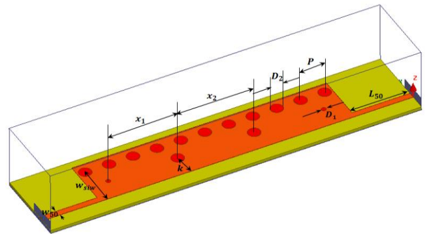
Fig. 14. Geometric design of HMSIW filter with Geometric design of SIW filter.
