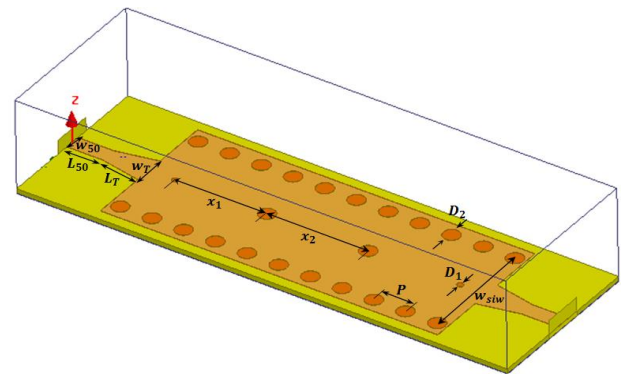
Fig. 5. Geometric design of the SIW filter using shunt-inductive posts for coupling
