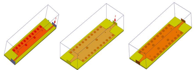
Fig. 1. The different proposed SIW/HMSIW bandpass filter designs
