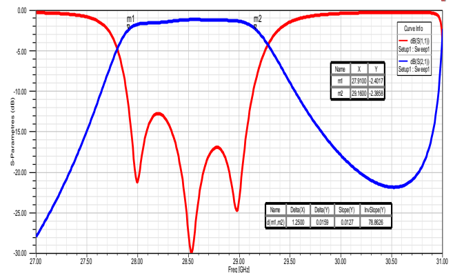
Fig. 6. S-parameters of the proposed SIW bandpass filter with initial geometric parameters
