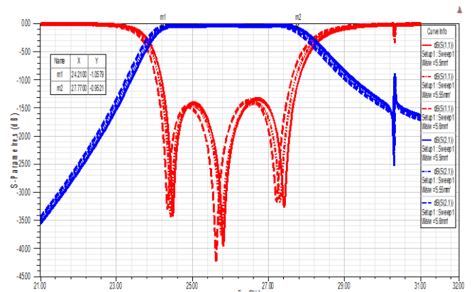
Fig. 16. S-Parameters of the new 3 rd SIW bandpass iris shunt inductive filter based on DGS technique
