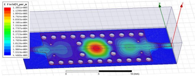
Fig. 11. Simulated E-field magnitude distributions obtained by SIW bandpass filter
