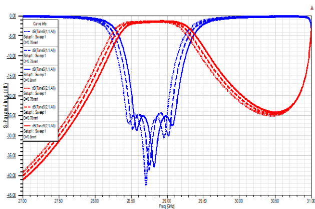
Fig. 13. Variation of the diameter D of the proposed bandpass filter SIW
