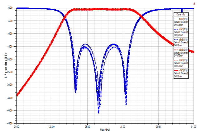
Fig. 15. S-Parameters of the proposed HMSIW bandpass filter with optimal geometric parameters
