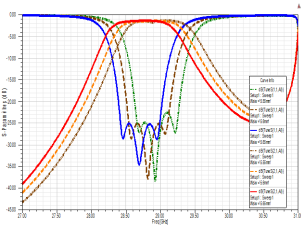
Fig. 12. W_SIW spacing varying effect for the proposed 3 rd SIW bandpass filter
