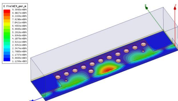
Fig. 17. Simulated E-field magnitude distributions obtained by SIW -DGS bandpass filter.
