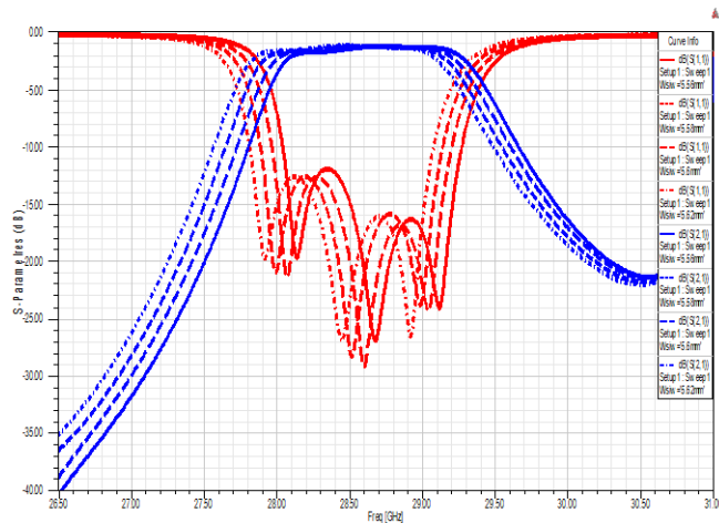
Fig. 7. W_{SIW} spacing variation effect for the proposed 3 rd SIW bandpass filter
