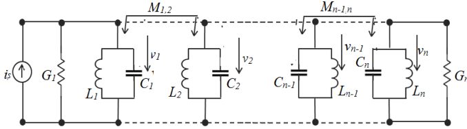
Fig. 2. Equivalent circuits of nth coupled resonators electric coupled resonators
