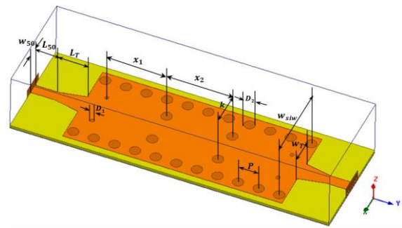
Fig. 9. Geometric design of the SIW filter using shunt-inductive iris for coupling
