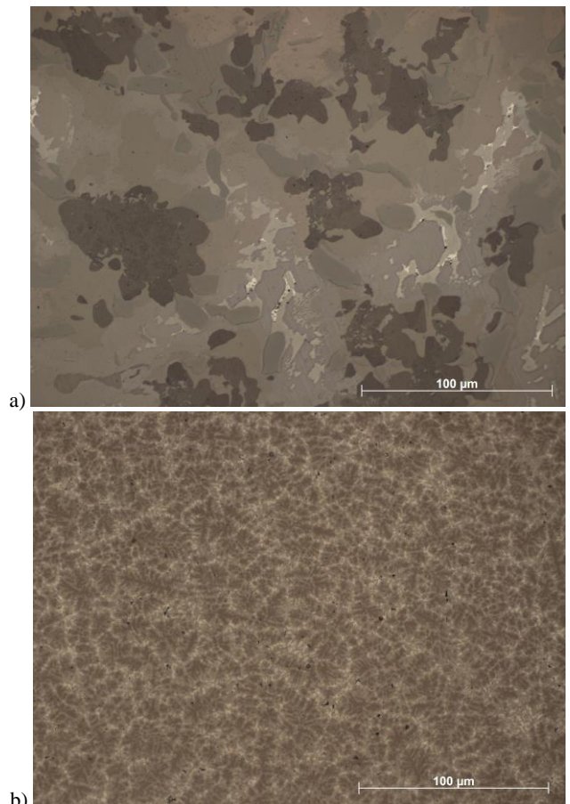
Fig. 4. Microstructure of Al_{71}Ni_{24}Fe_5 alloy in a form of a) ingot, b) plate
