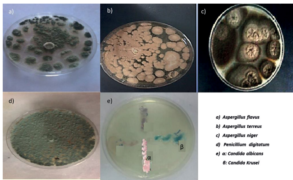
Photo 1. Fungi isolated from wastewater treatment plant: a) Aspergillus flavus , b) A. terreus , c) A. niger , d) Penicillium digitatum , e) \alpha : Candida albicans , and \beta : C. krusei (phot. I.M. Al Hussaini)
