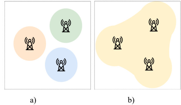
Fig. 1. Coverage obtained in the multi-frequency network (a) and in the single-frequency network (b)
