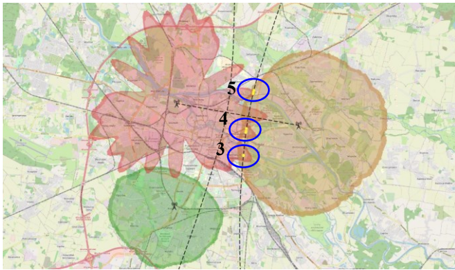
Fig. 9. Designated measuring locations for WUST – NIT route, n = 950 , \Delta d = 1\,313.11 m.
