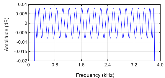
Fig. 4. Passband amplitude ripples for B_r=4.5\% and N=82 .
