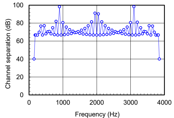
Fig. 5. Channel separation performance for analogue signal.
