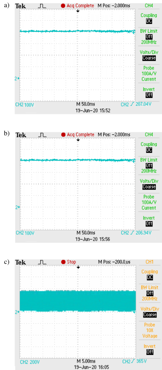
Fig. 8. a) capacitor 1 voltage, b) capacitor 2 voltage, c) Z-source network output voltage
