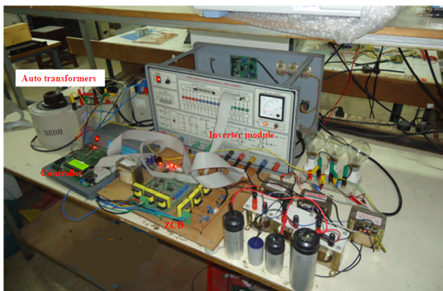
Fig. 3. ZSI-UPQC experimental set-up
