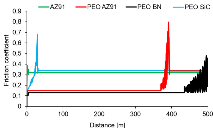
Fig. 4. The friction coefficient as a function of the sliding distance for the AZ91 magnesium alloy (without or with a coating) – steel 1.3505 rubbing pair, using a rotational speed of 0.02 m/s
