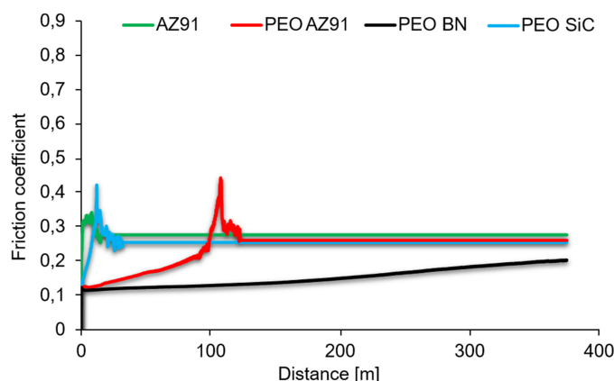
Fig. 5. The friction coefficient as a function of the sliding distance for the AZ91 magnesium alloy (without or with a coating) – steel 1.3505 rubbing pair, using a rotational speed of 0.2 m/s
