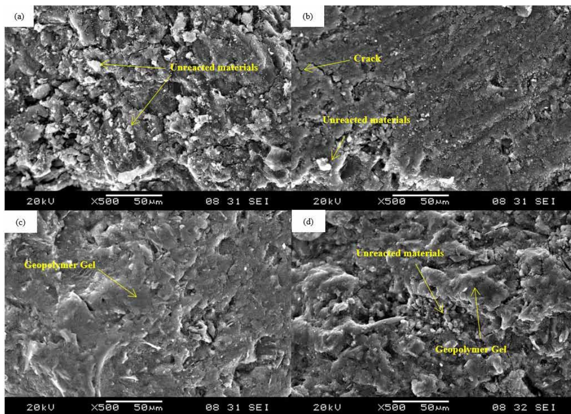
Fig. 3. The morphology of metakaolin/dolomite geopolymer for different solid to liquid ratio (a) 0.4, (b) 0.6, (c) 0.8 and (d) 1.0
