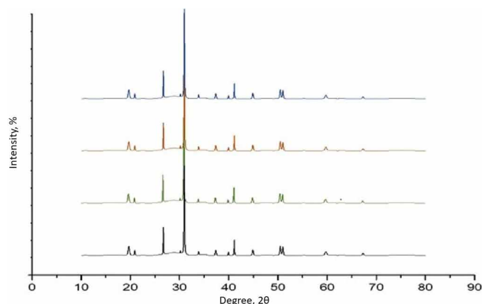
Fig. 1. Phase analysis of the metakaolin/dolomite geopolymer
