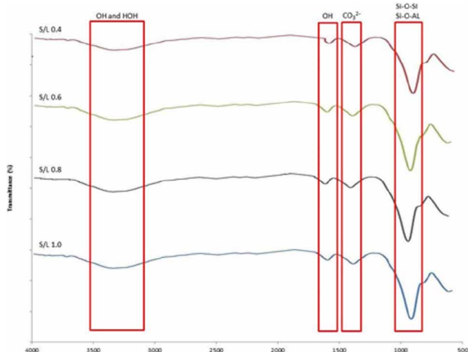
Fig. 4. FTIR spectrum of metakaolin/dolomite geopolymer with different S/L ratio
