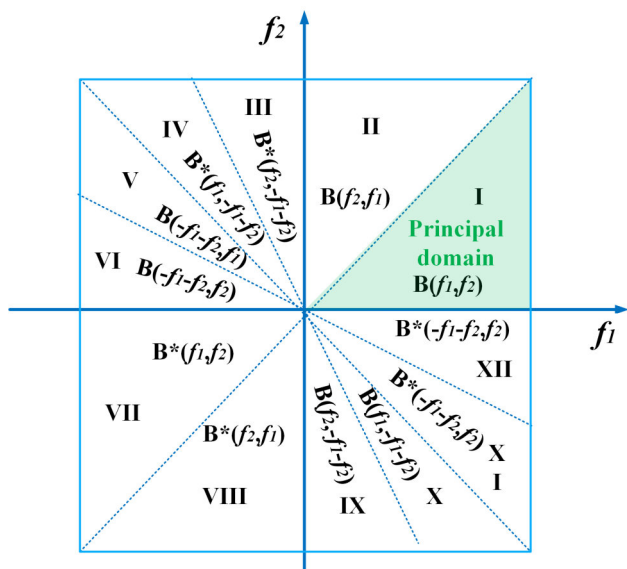
Fig. 1. Bispectrum symmetry regions
